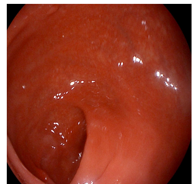
[8]Sigmoid Colon
