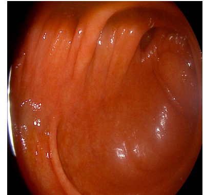
[4]Ascending Colon
