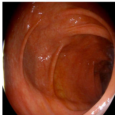
[5]Hepatic flexure
