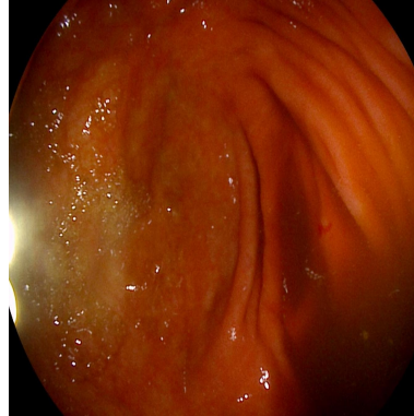
[1]Appendiceal Orifice
