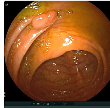
[2]Ascending Colon
