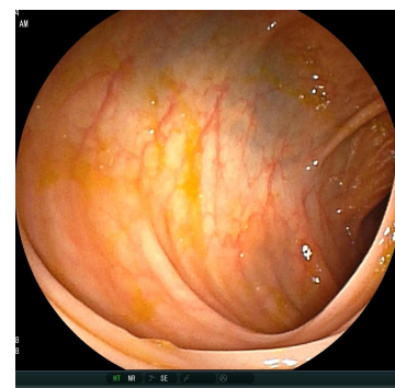
[8]Splenic flexure
