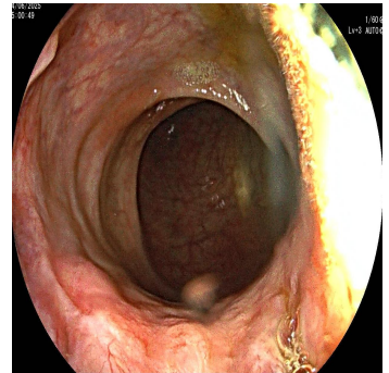
[16] Anal canal
