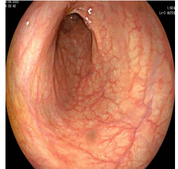
[12] Descending Colon
