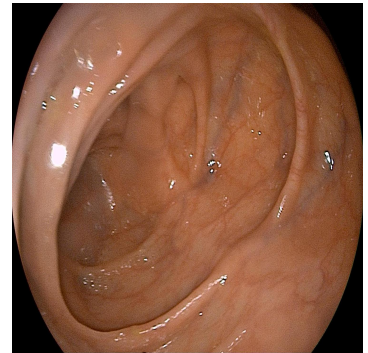
[4]Hepatic flexure
