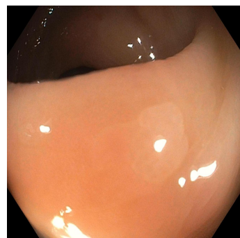
[20] Sigmoid Colon
