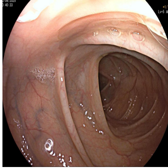
[10] Ascending Colon
