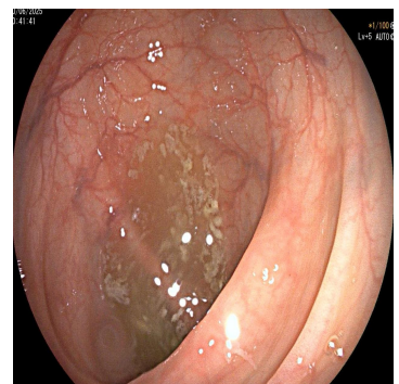
[8]Hepatic flexure
