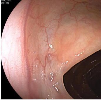
[9] Ascending Colon
