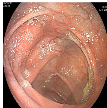
[4]Transverse Colon
