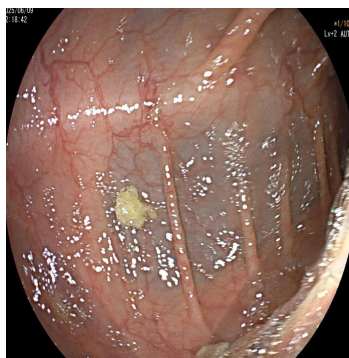
[3]Hepatic flexure
