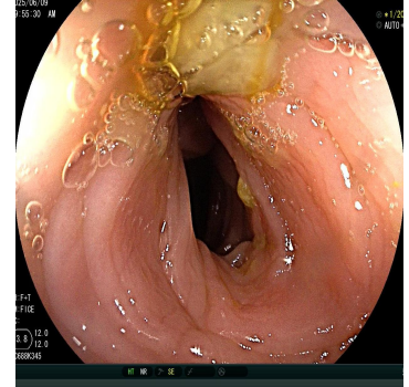
[2]Hepatic flexure
