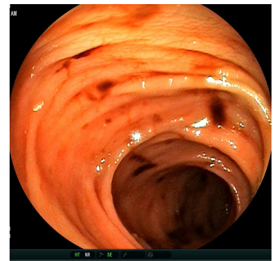
[6]Descending Colon
