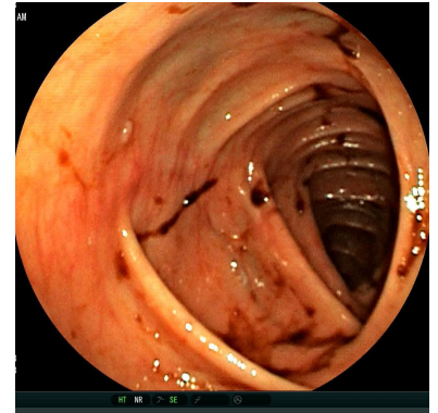
[4]Splenic flexure
