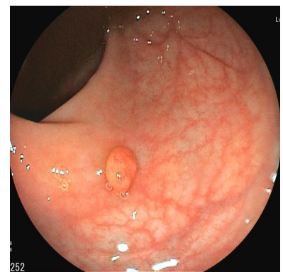
[8]sigmoid
