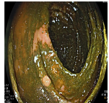
[6]Ascending Colon
