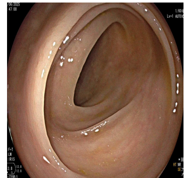
[8]Splenic flexure
