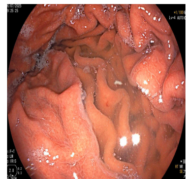
[8]Body
