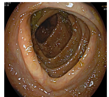
[2]Ascending Colon
