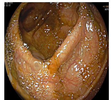
[1]Cecum
