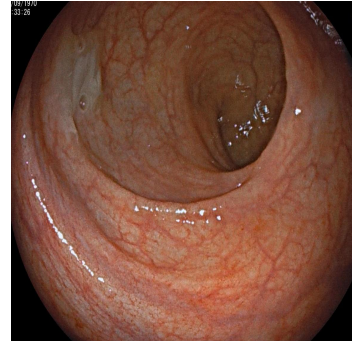
[8] Rectum
