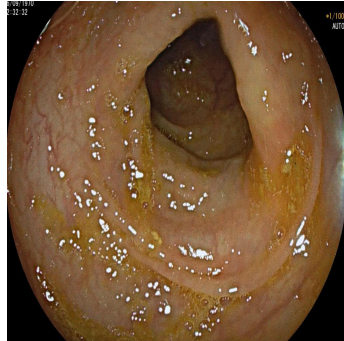
[6] Descending Colon
