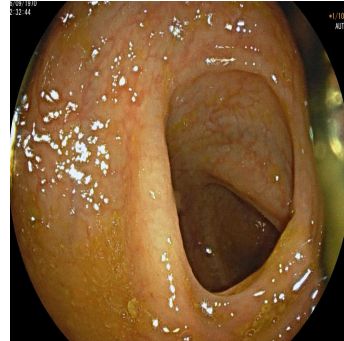
[7] Sigmoid Colon
