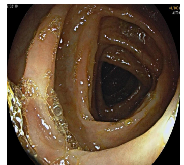
[3]Hepatic flexure
